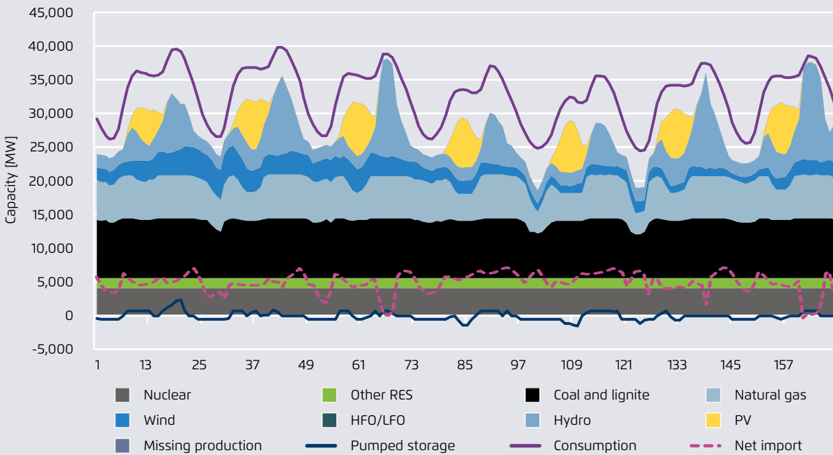
Electricity generation and demand in the SEE region for the critical autumn week in 2030, MW
