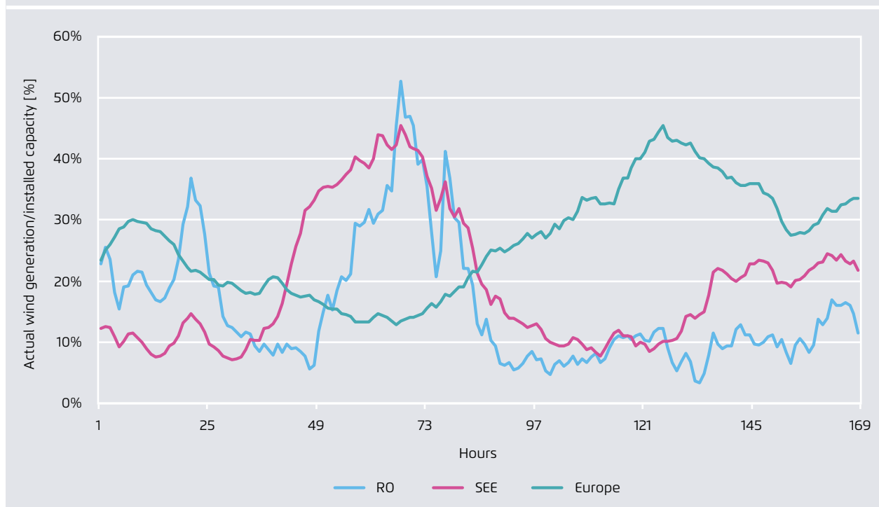
Time series of onshore wind power generation in a simulation for the first week of 2030 at different levels of aggregation
