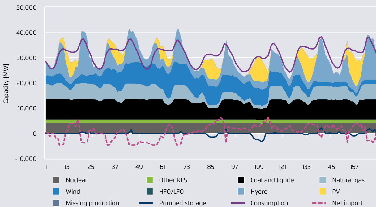
Electricity generation and demand in the SEE region for the critical spring week in 2030, MW
