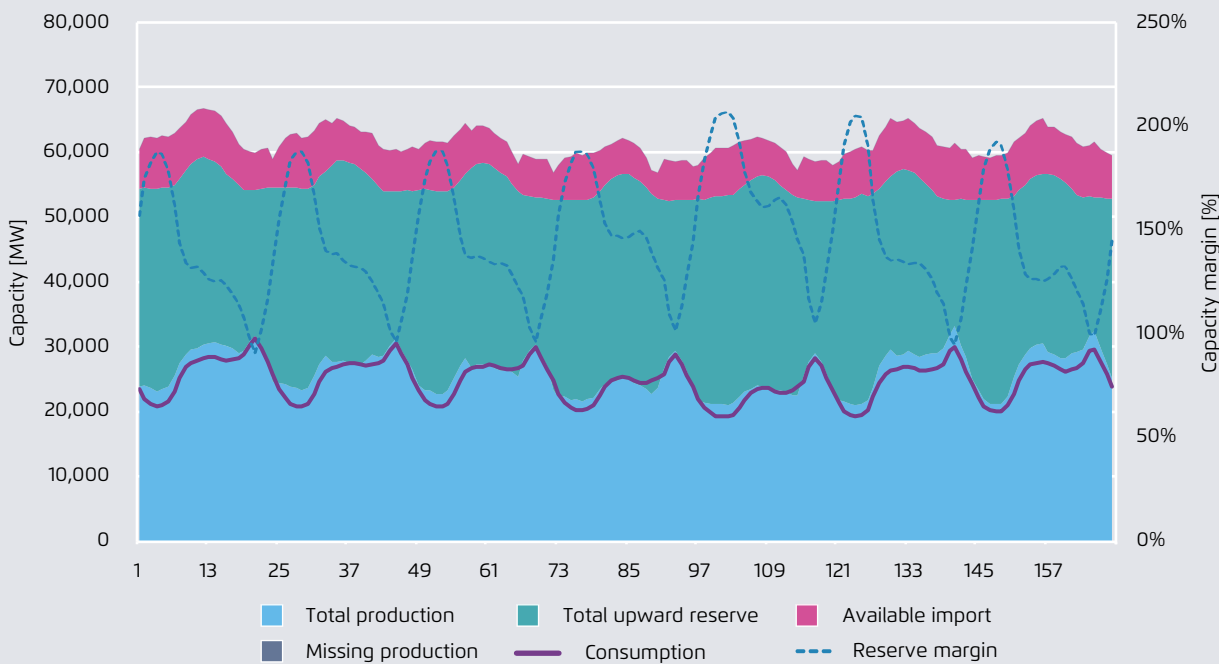
Reserve margin in the SEE region for the critical summer week in 2017, MW
