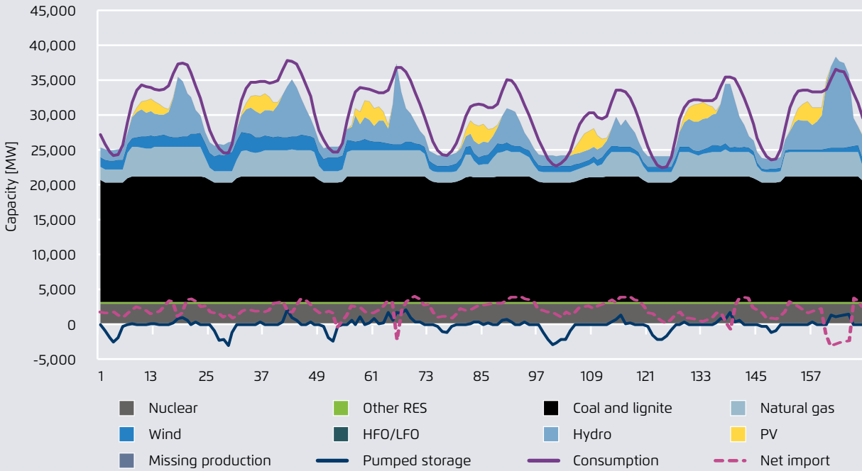
Electricity generation and demand in the SEE region for the critical autumn week in 2017, MW
