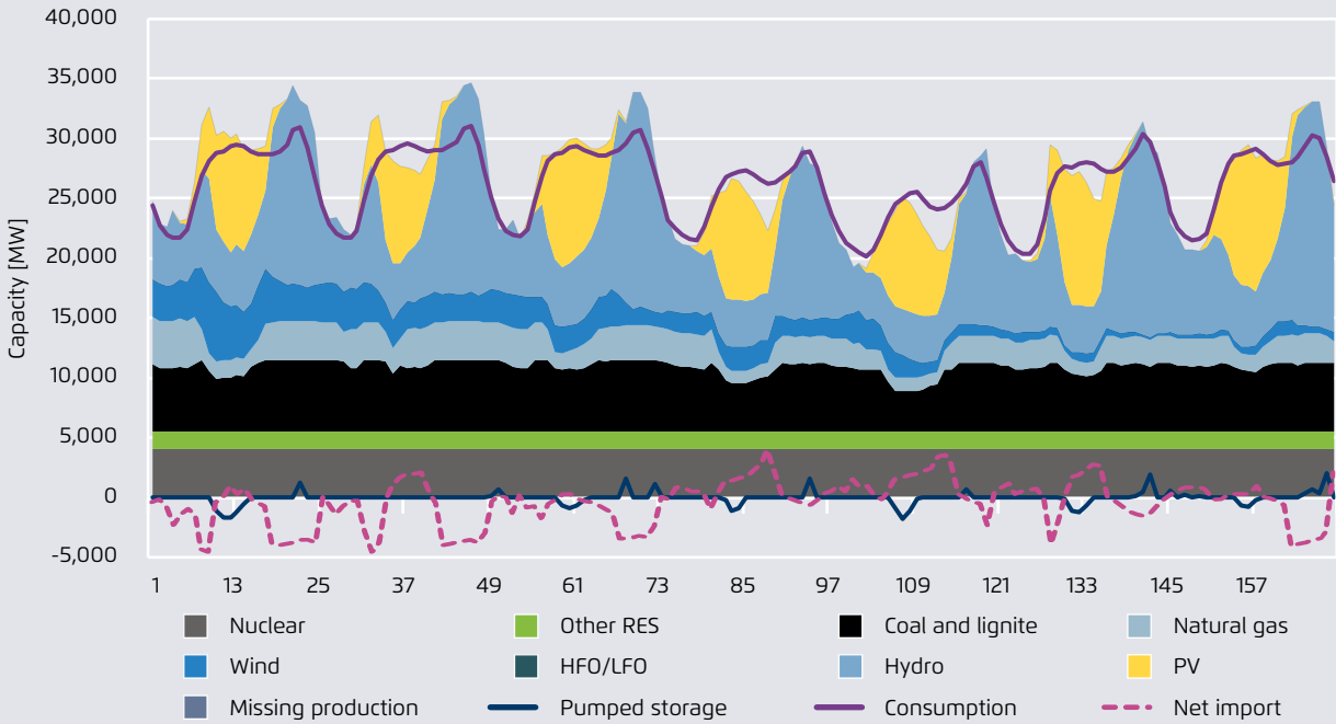
Electricity generation and demand in the SEE region for the critical summer week in 2030, MW
