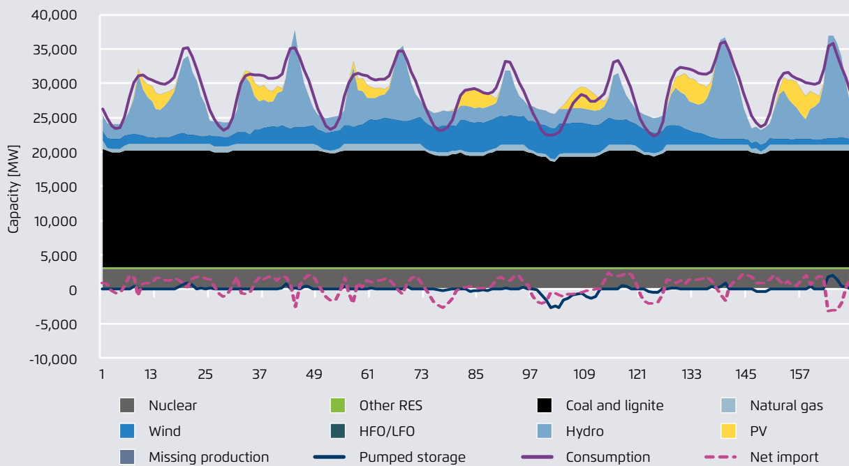
Electricity generation and demand in the SEE region for the critical spring week in 2017, MW
