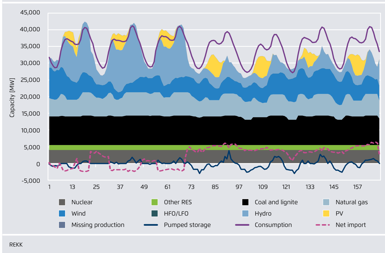
Electricity generation and demand in the SEE region for the critical week in winter in 2030 in MW Figure ES 5
